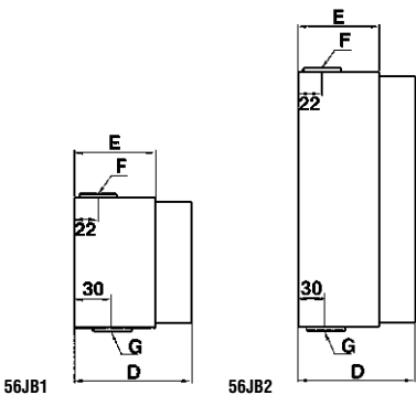
Dimensional Drawings
